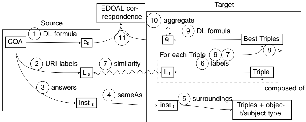
Figure 3.2: Schema of the general approach (from [Theblin et al., 2018c]).
