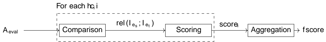
Figure 6.4: Evaluation process for intrinsic instance-based precision
