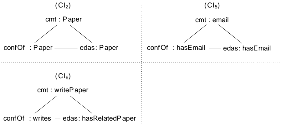
Figure 4.2: Cliques found by the proposed holistic approach.
