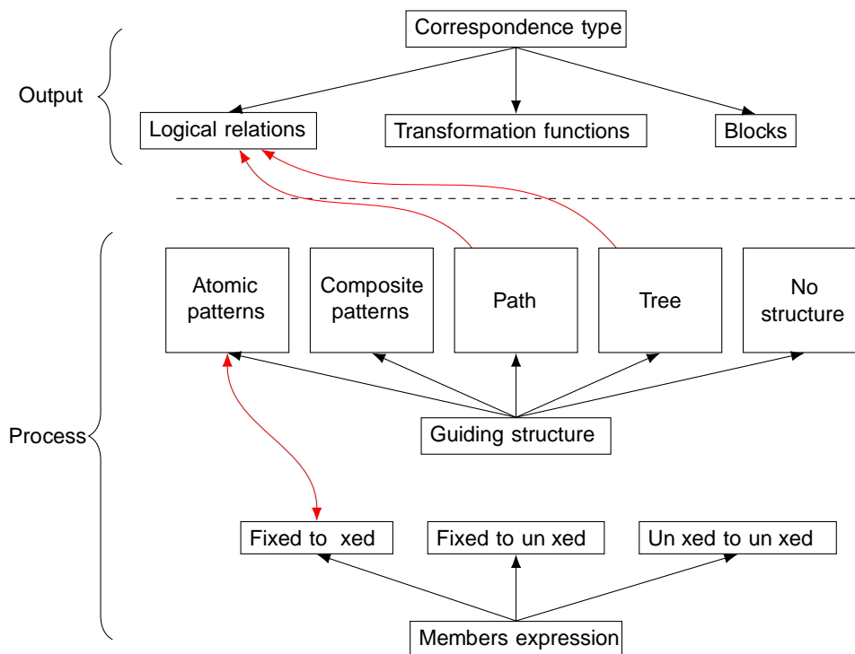
Figure 3.1: Two axes to characterize the complex matching approaches: output and process. The correlation between the categories are represented with red arrows (from [Theblin et al., 2019c]).
