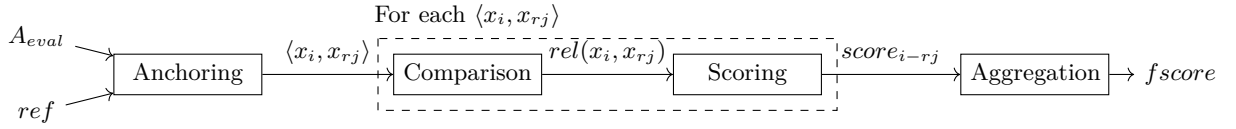
Figure 6.2: Evaluation process of the alignment A_{eval} with a reference ref .
