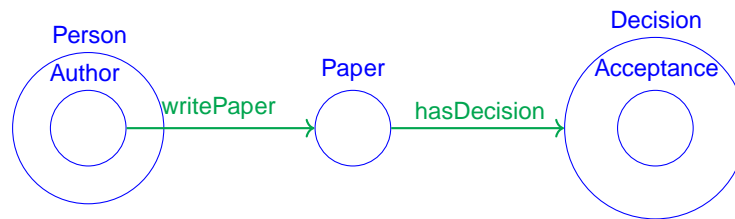
Figure 2.3: Fragment of cmt ontology.
