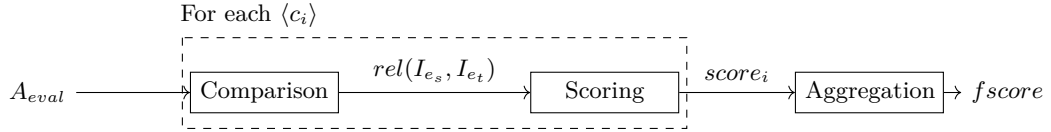
Figure 6.4: Evaluation process for intrinsic instance-based precision
