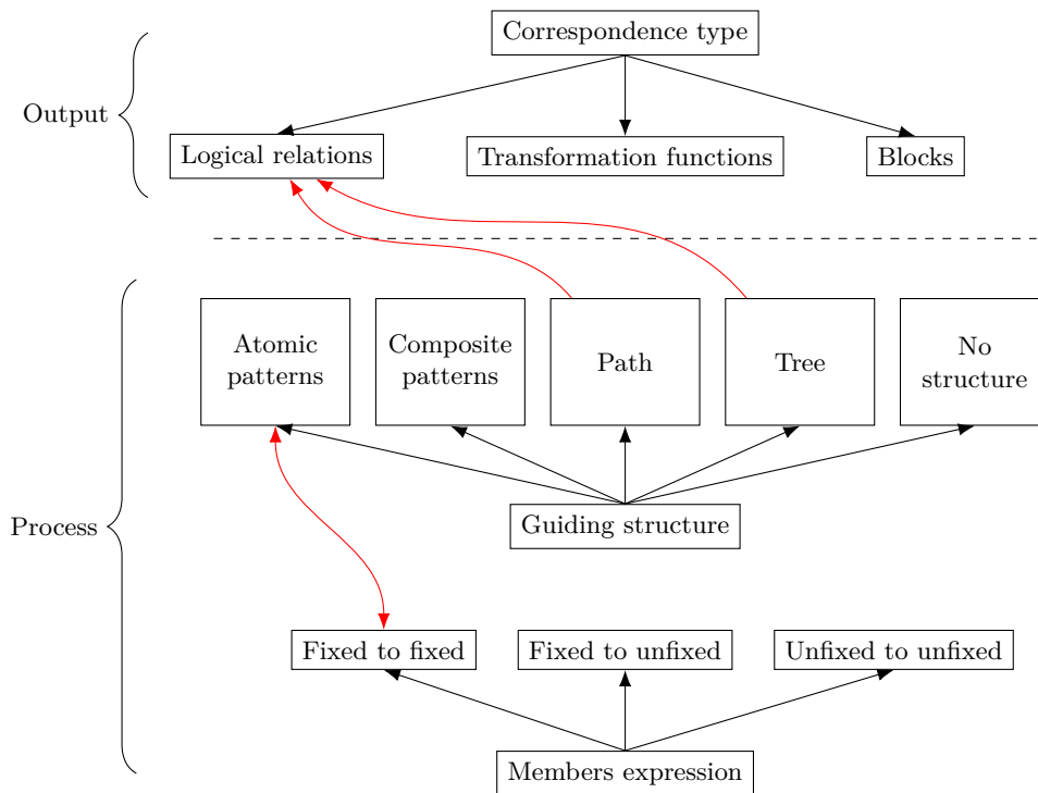
Figure 3.1: Two axes to characterize the complex matching approaches: output and process. The correlation between the categories are represented with red arrows (from [Thiéblin et al., 2019c]).
