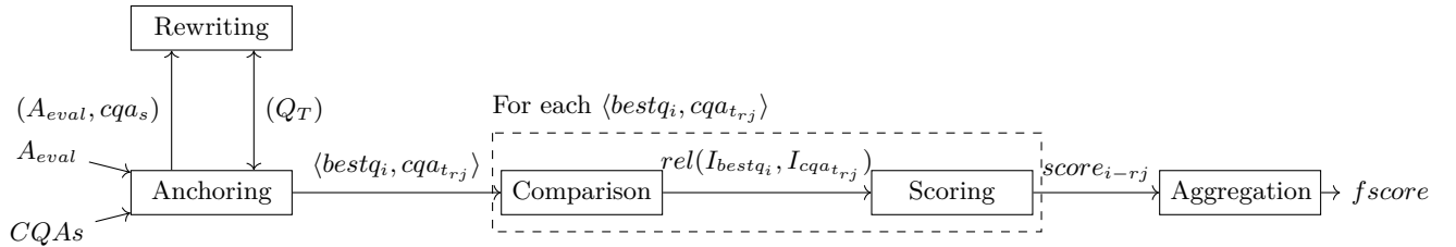
Figure 6.3: CQA-coverage evaluation process.
