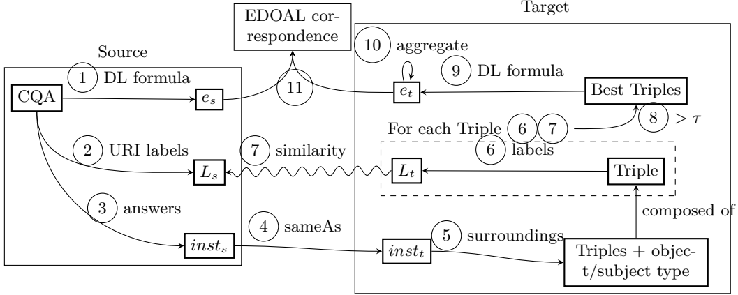
Figure 3.2: Schema of the general approach (from [Thiéblin et al., 2018c]).
