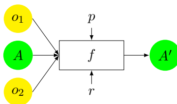
Figure 2.1: The matching process (adapted from [Euzenat and Shvaiko, 2013] (page 41)).
