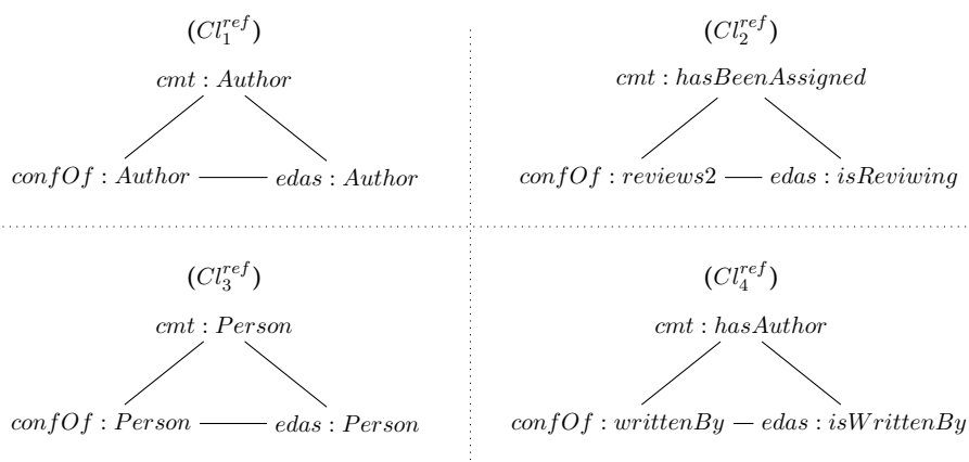
Figure 4.1: Reference cliques (Cl_1^{ref}) , (Cl_2^{ref}) , (Cl_3^{ref}) , and (Cl_4^{ref}) .
