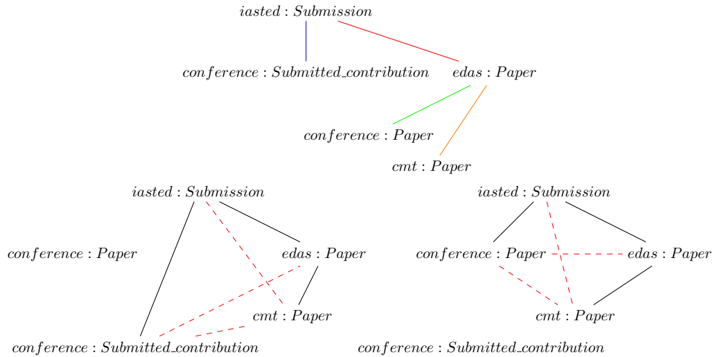
Figure 7.4: (a) Original extracted subgraph (top), (b) method 1 (left), (c) method 2 (right).
