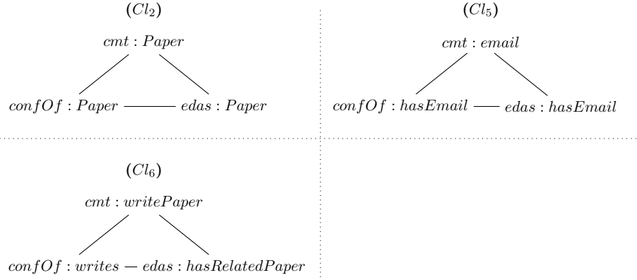
Figure 4.2: Cliques found by the proposed holistic approach.
