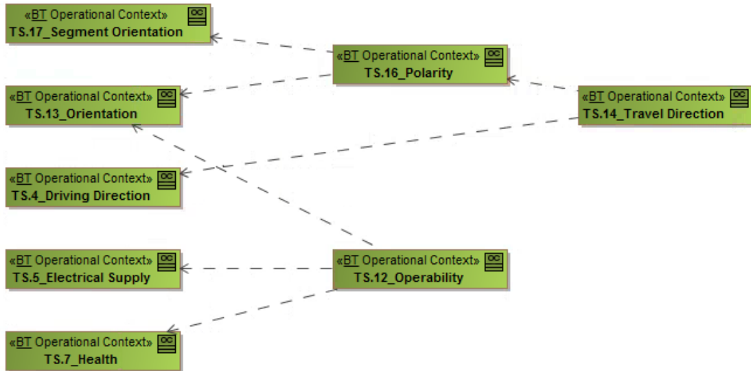
Figure 6.3: Dependencies between train types of states
