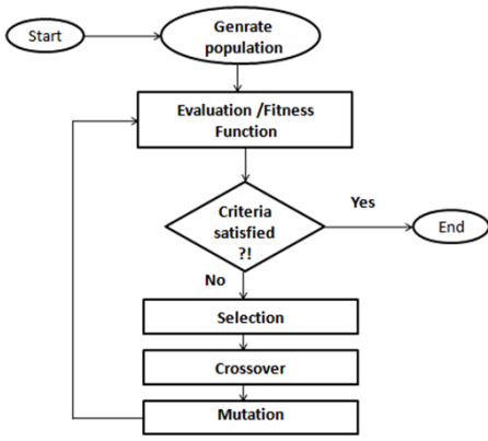
Fig. 2. Flowchart of the standard GA steps
