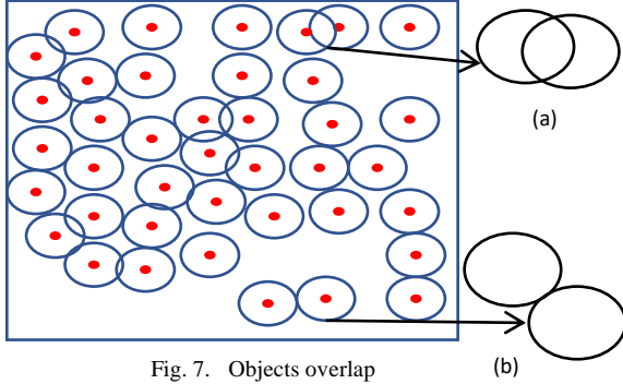
Fig. 7. Objects overlap
