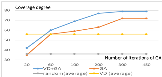
Fig. 13. Comparing the coverage degree according to the Number of iterations for VD, GA and VD-GA
