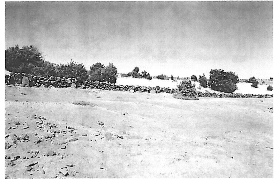
Figure 7.3 Ait Inzal cemetery under agdal prohibition with an obvious result on the herbaceous and Juniperus oxycedrus (pool of biodiversity and seed distribution point) (based on Domínguez, 2010)
