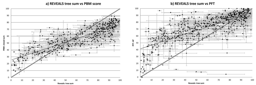
Figure 3. Major axis regression between forest cover estimates for different pollen-based methods by grid cell; (a) REVEALS tree sum vs PBM score; (b) REVEALS tree sum vs PFT.
