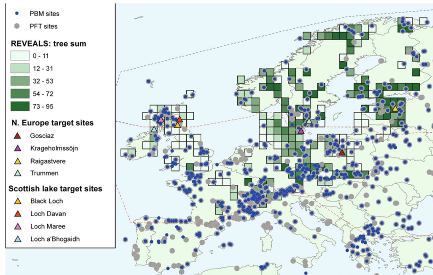
Figure 1. Map of Europe showing sub-divisions used, and grid cells map for mid-latitude (mixed temperate forest zone) and northern (boreal needle-leaf forest zone) Europe. [map generated using ArcMap (version: 10.4) URL: http://desktop.arcgis.com/en/arcmap/ ].
