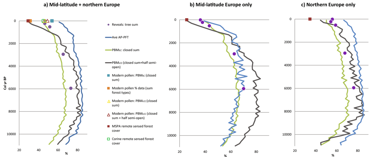
Figure 2. Pollen-inferred forest cover for mid-latitude and northern Europe during the last 11,000 years (REVEALS grid cells only).
