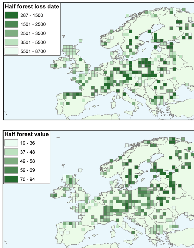
Figure 4. Mapped regional differences in timing of forest loss in calendar years BP. PBM_{sc} by grid cell for “half-life” (i.e. date of half-way point between forest cover maximum and minimum). [map generated using ArcMap (version: 10.4) http://desktop.arcgis.com/en/arcmap/ ].
