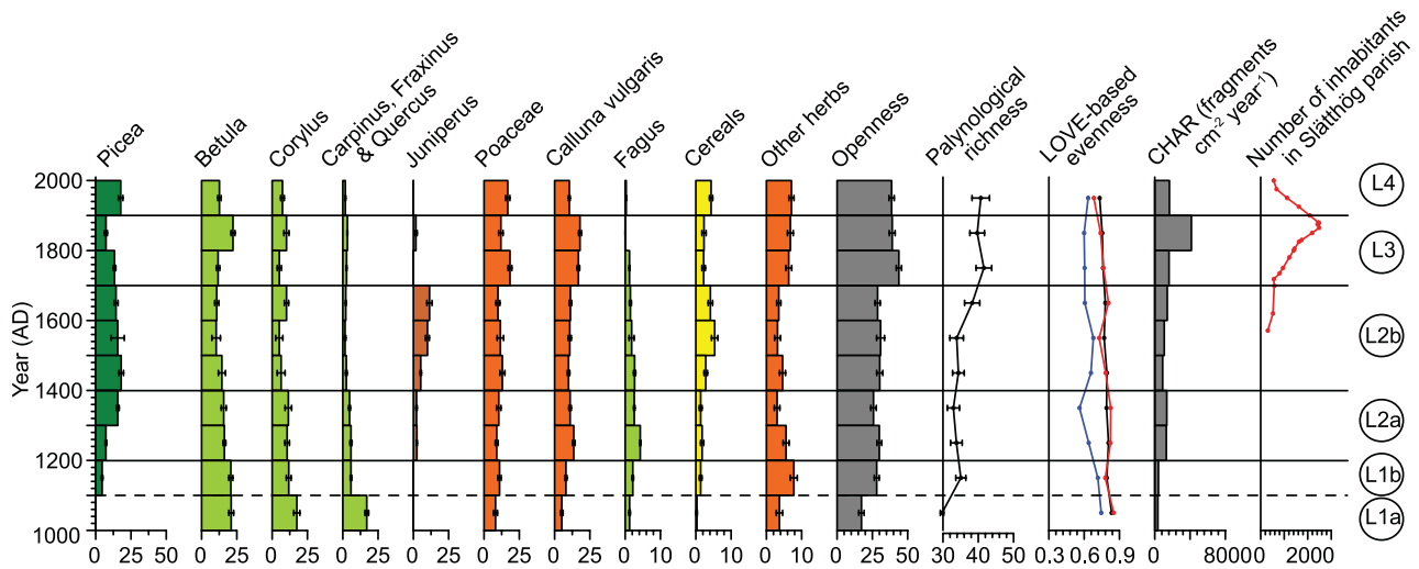
Figure 5. Lake Lindhultsgöl. Estimates of local vegetation cover for selected taxa/taxa groups, openness, palynological richness, LOVE-based evenness, charcoal accumulation rate (CHAR) and population in Slätthög parish. Cereals include both Cerealia type and Secale type. Openness includes all herb taxa and Calluna vulgaris . LOVE-based evenness was calculated for all 26 reconstructed taxa (black line), trees (red line) and herbs (blue line) taxa. We divided the sequence into four major land-use periods (L1–L4).
