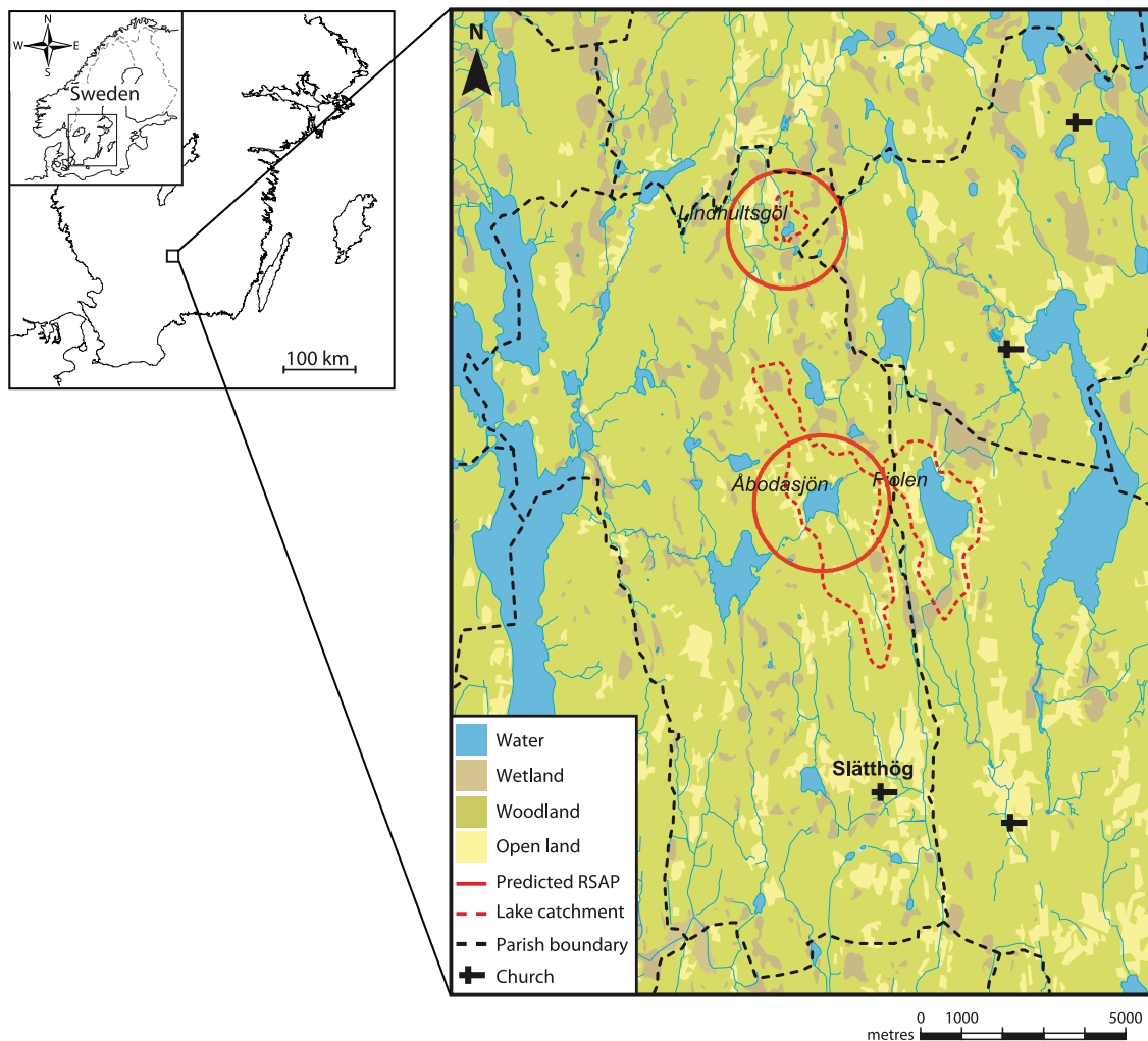
Figure 1. Locations of Lakes Fiolen, Åbodasjön and Lindhultsgöl in southern Sweden. Red circles show the predicted relevant source area of pollen (predicted RSAP) around Åbodasjön and Lindhultsgöl, 1740 and 1440 m, respectively (Mazier et al., 2015). Parish boundaries (black dashed lines), catchments for the respective lakes (red dashed lines) and the modern land-cover are also shown.
