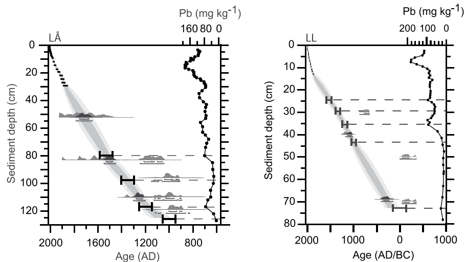
Figure 7. Lake Åbodasjön (LÅ) and Lake Lindhultsgöl (LL). Age–depth models based on ^{210}\text{Pb} records (horizontal bars), calibrated radiocarbon dates obtained on terrestrial macrofossils, ^{210}\text{Pb} dates and Pb pollution marker horizons (thick horizontal bars), along with the respective records of total Pb concentration. Depths of pollution marker horizons are marked by the dashed lines. The modelled \pm 1\sigma and \pm 2\sigma confidence intervals are marked by dark grey and grey shading, respectively.
