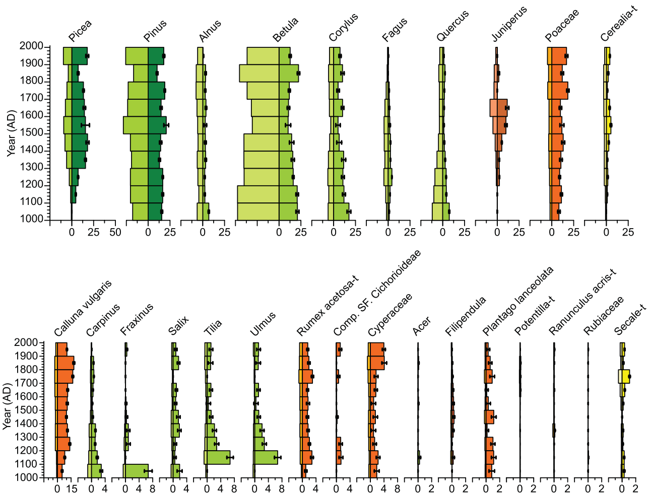
Figure 3. Lake Lindhultsgöl. Pollen percentage diagram (left side) and estimated local vegetation proportions within RSAP (right side) at 100-year time windows for 26 taxa, based on pollen analysis and the LOVE model. Note the different scales for the upper and lower parts of the figure, and within the lower figure.
