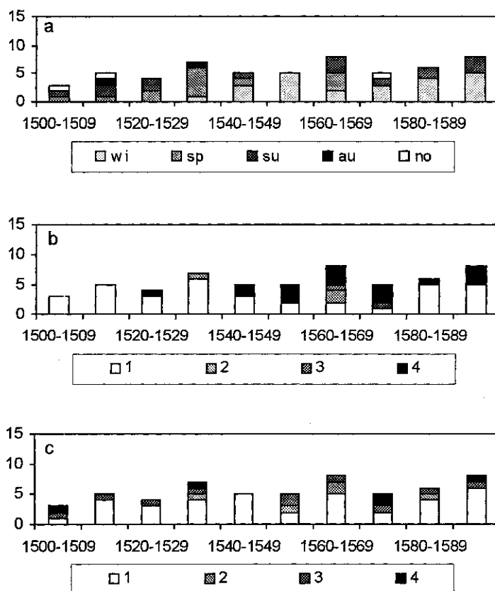
Figure 12. Decennial frequencies of floods on the middle Elbe with an indication of seasonality (a), their causes (b) and class of damage (c) during the sixteenth century. Explanation see Figure 10.
