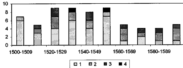
Figure 17. Decennial severity and scale extension of floods in northern and central Italy during the sixteenth century. Explanation: 1 - local, 2 - regional, 3 - large-scale or only one isolated catastrophe, 4 - large-scale and more than one catastrophe.
