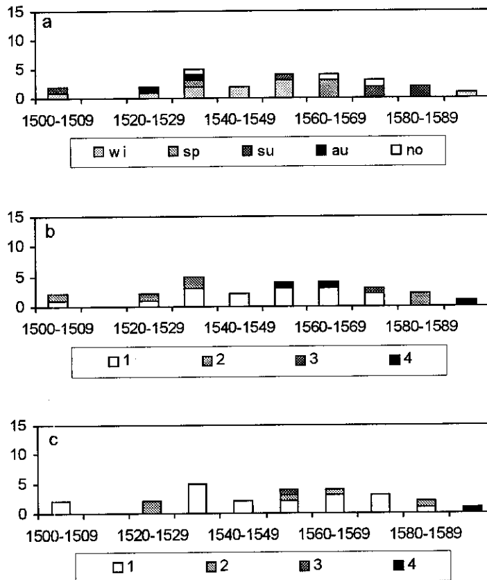
Figure 13. Decennial frequencies of floods on the Saale with an indication of seasonality (a), their causes (b) and class of damage (c) during the sixteenth century. Explanation see Figure 10.
