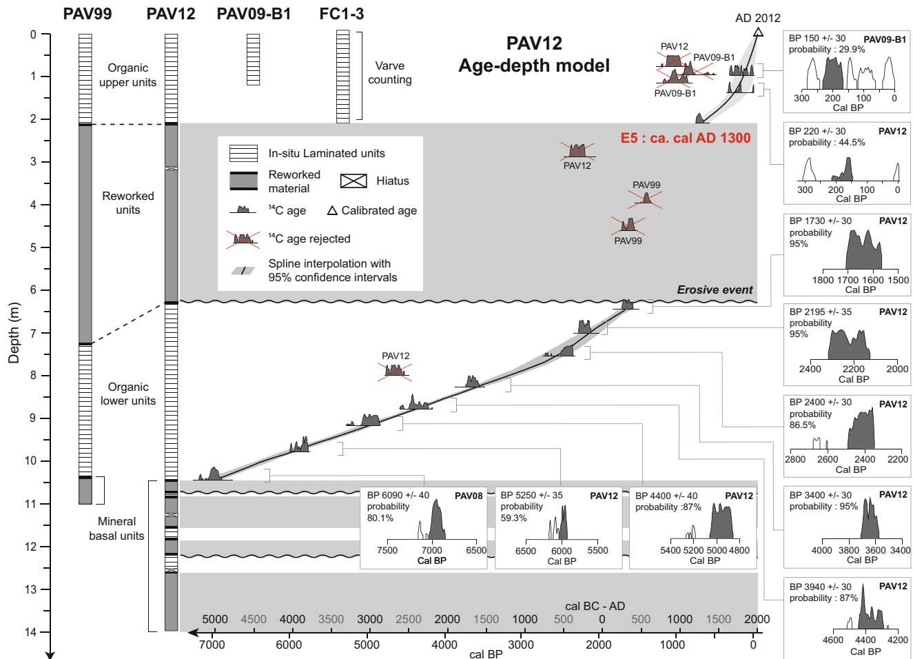
Fig. 23.6 Age depth model of core PAV12 based on AMS radiocarbon ages from organic macro remains using the Intcal09 calibration curve from Reimer et al. (2013), the identification of reworked deposits intercalated within the central basin fill and the application of a spline interpolation between the dating points using the CLAM software (Blaauw
