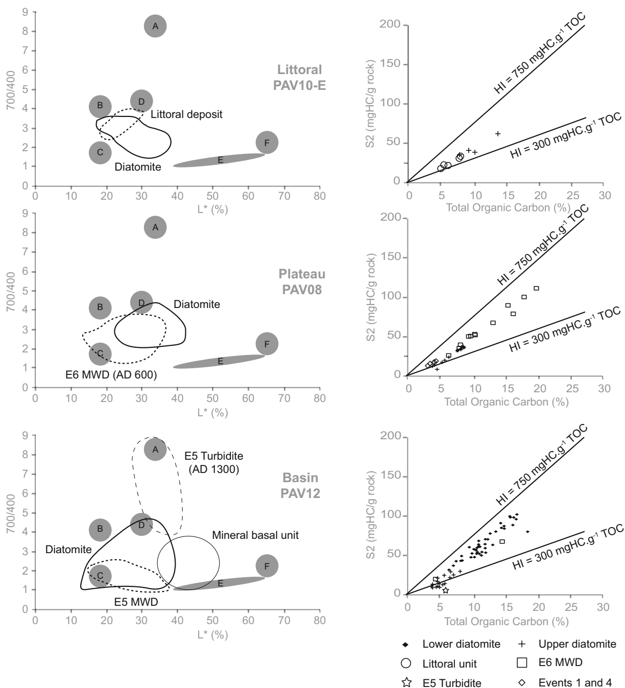
Fig. 23.9 Characterization of Pavin sediments origin and sediment source based on diffuse spectral reflectance Q7/4 diagram (left) and Rock-Eval pyrolysis represented by S2 vs. TOC diagram (right) for cores PAV10-E (littoral), PAV08 (plateau) and PAV12 (basin). In the Q7/4 diagram, the diffuse spectral reflectance signature of littoral deposit, diatomite, Mass-Wasting Deposit (MWD), Turbidite and Mineral Basal unit are compared to the five distinct poles of sediments defined by Debret et al (2011): Iron-Rich deposits (a); Organic-rich
