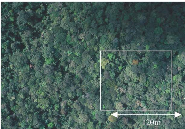
Photo 1. View of forest canopy at three scales on plot P11, Paracou. Original scales of the slides, from the bottom up, are: 1:8000; 1:3000; 1:1500. Photographs, D. Guillemyn.
