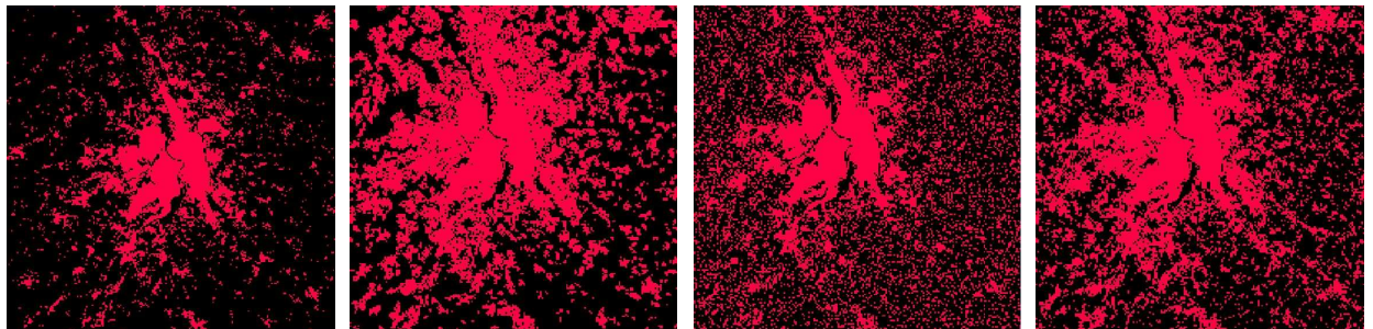
Figure 3: Built-up areas in 2006 and urban growth simulations by 2100 based on compact, sprawling and combined patterns.
