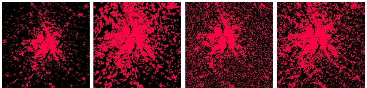
Figure 3: Built-up areas in 2006 and urban growth simulations by 2100 based on compact, sprawling and combined patterns.
